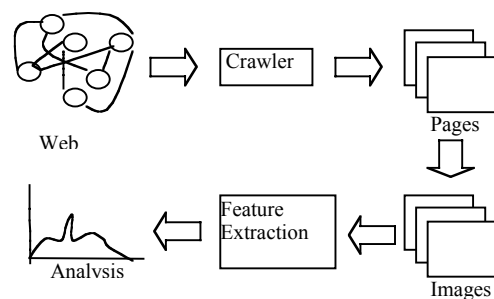
Fig. 1. Overall architecture.
