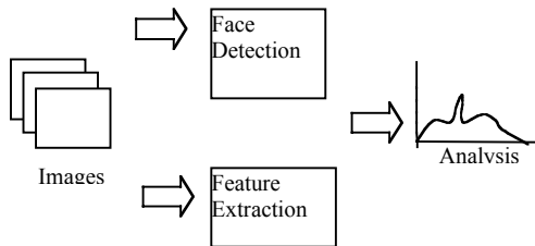
Fig. 2. Content-based analysis.
